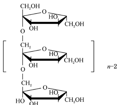
Figure 2 -- Schematic diagram of the molecular structure of fructose-fructose (F n ) fructooligosaccharides
