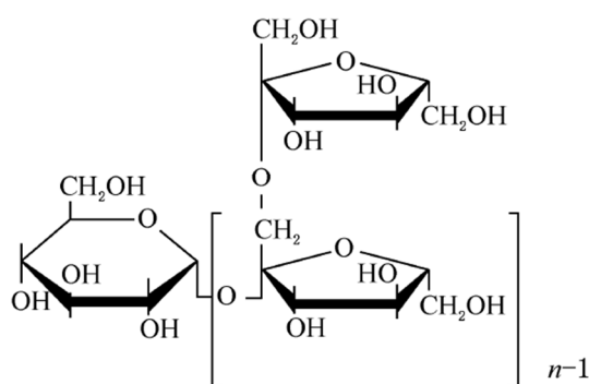
Figure 1 -- Schematic diagram of the molecular structure of sucrose-fructose (GF n ) fructooligosaccharides
